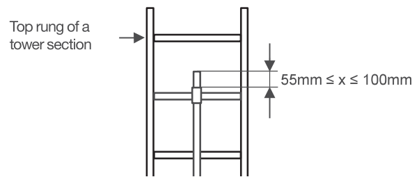
Length limits of the top and bottom ends of the safety rail
